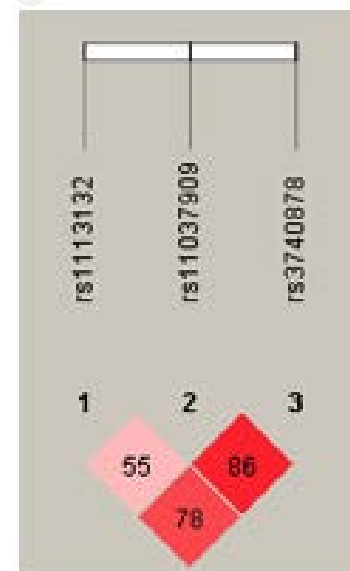
Figure 1. Linkage disequilibrium of EXT2 polymorphisms.
