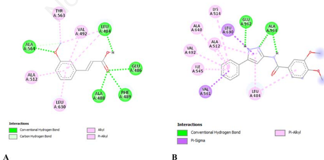
Figure 1. Interaction tested compounds (3MPCA (A) and native ligand (B)) with amino acids residue of protein FGFR-1.
