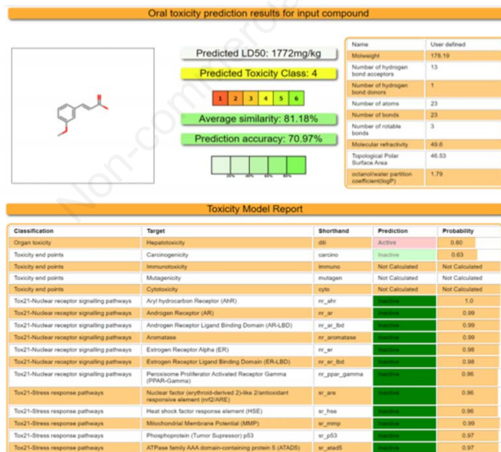
Figure 3. Toxicity prediction of 3MPCA using ProTox II online program.
